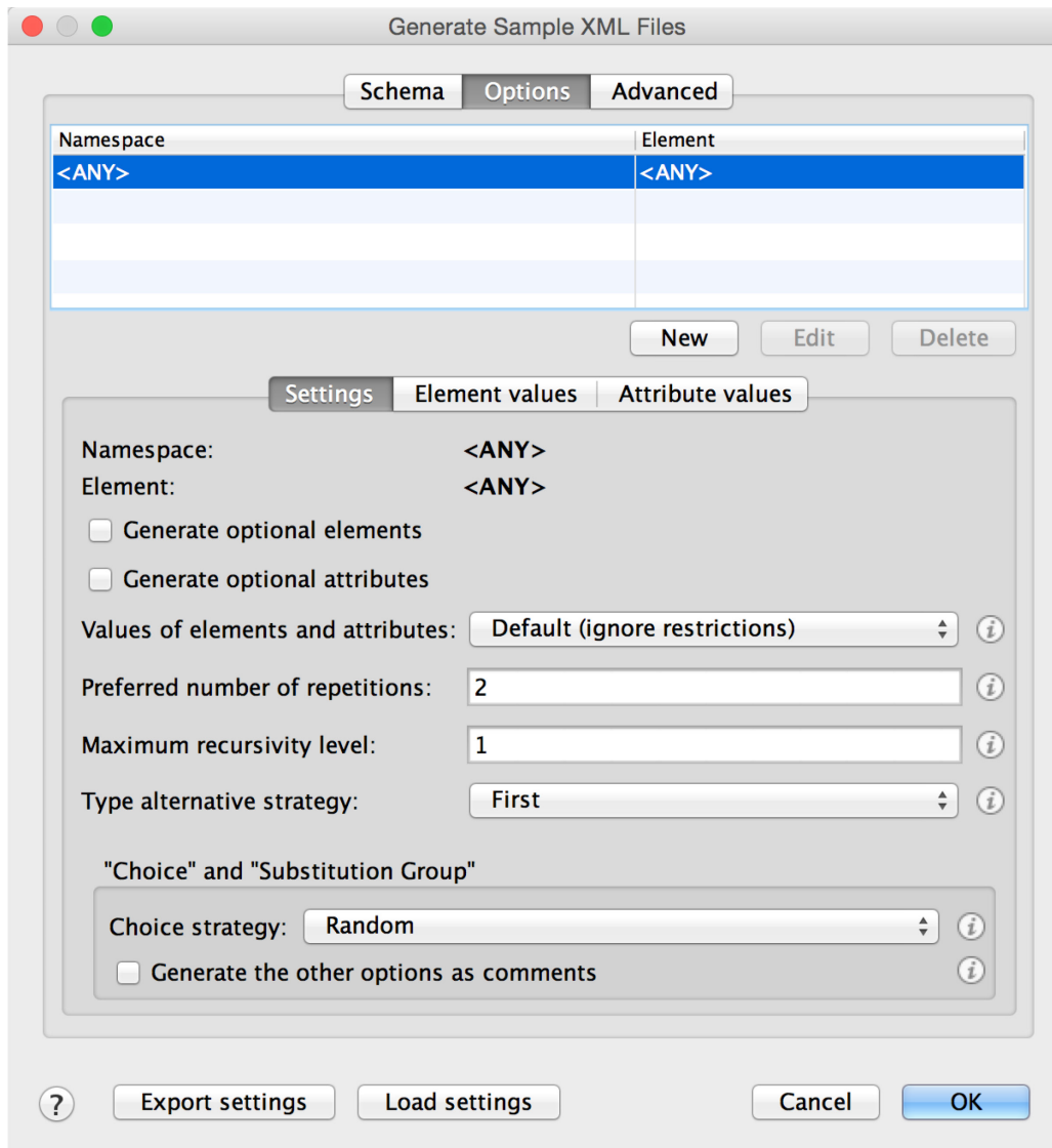
Figure D-9. Using oXygen to Generate an XML Label, part 2
