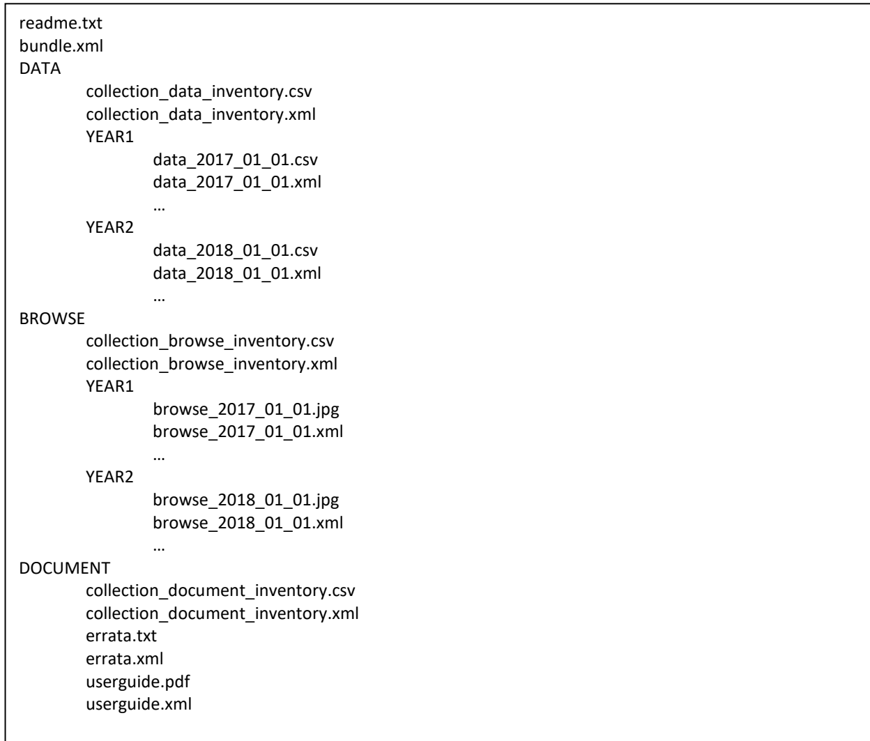
Figure 10-1. Example Archive Directory Structure
