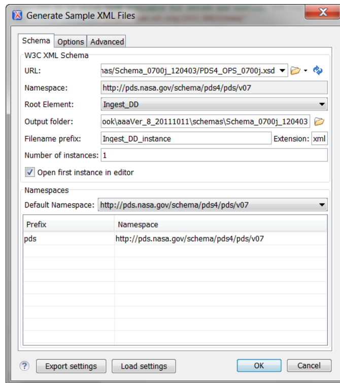
Figure J-2. Using oXygen to Generate a Label Template
