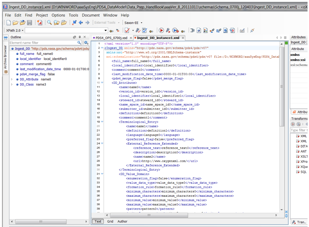
Figure J-3. Template input file for LDDTool as generated by oXygen
